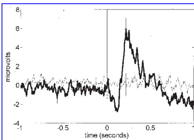
FIG. 4. Median electroencephalographic signals for the 7 male sessions combined.
